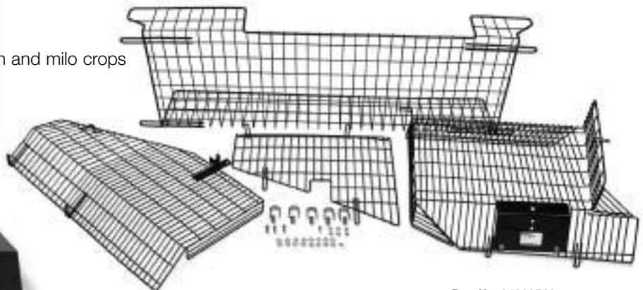
Part No. 84083562
