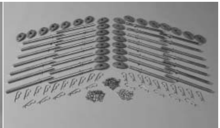
Part No. B96520 Auger Finger Complete Repair Kit
